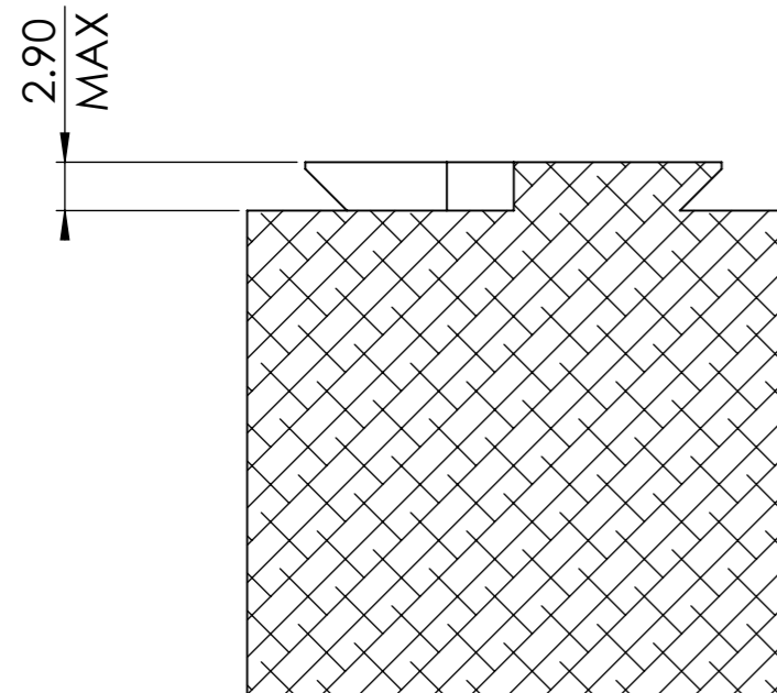
SECTION Z-Z
