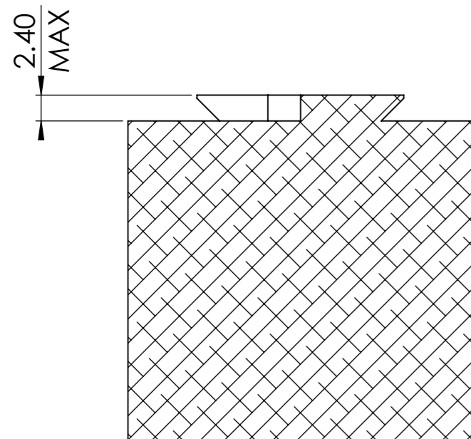
SECTION Z-Z
