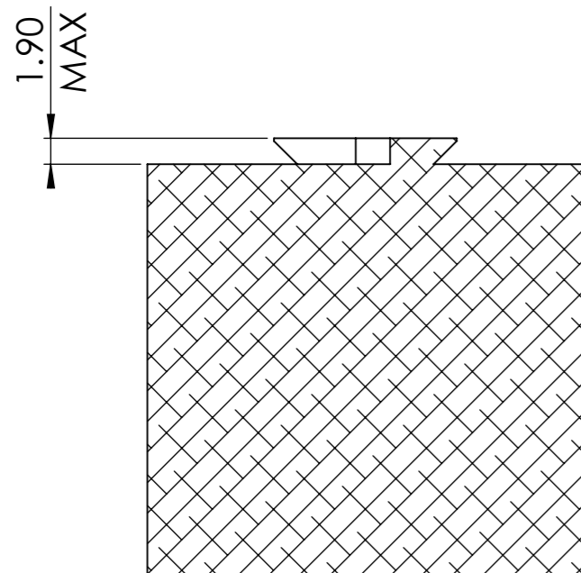
SECTION Z-Z
