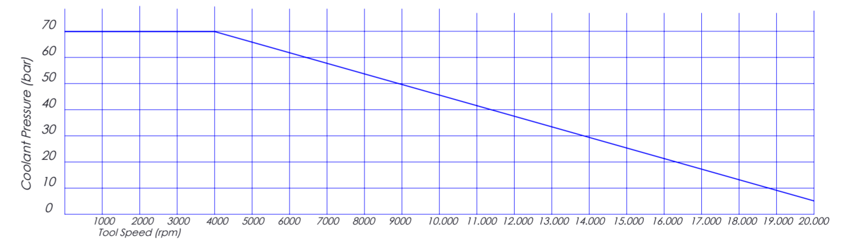
Coolant Pressure Variation
