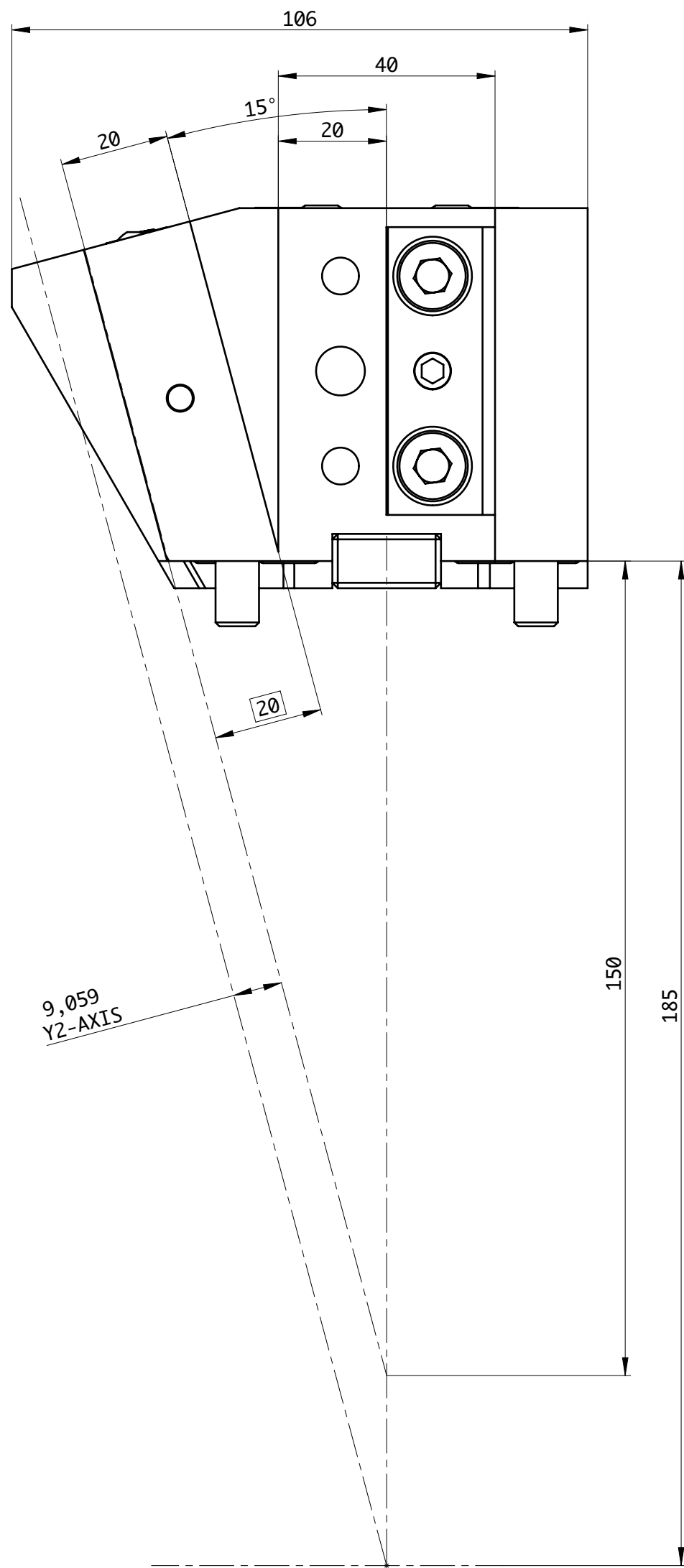
LOWER TURRET
