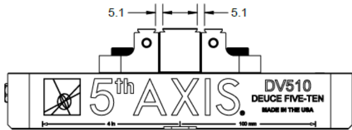
FORWARD JAWS (MINIMUM CLAMPING RANGE)
